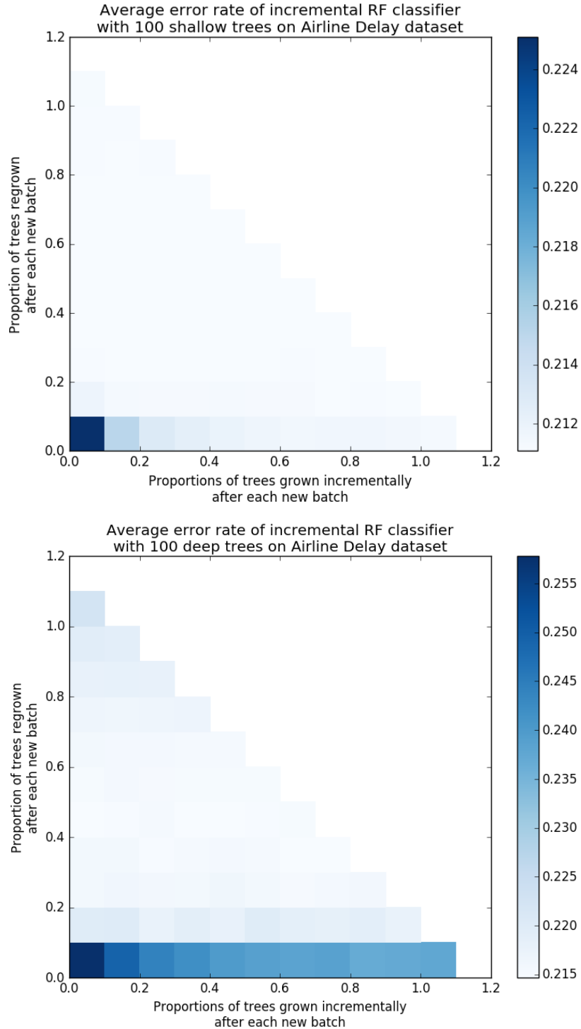
Figure 4-8: These two plots show the average error rates of various hybrid tree replacement and incremental growth strategies on the Airline Delay batched dataset. The axes indicate the percentage of trees that are modified according to each strategy.
