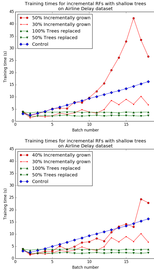
Figure 4-7: These graphs show the training times for the incremental growth strategy, the tree replacement strategy, and the control setting on the batched Airline Delay dataset.
